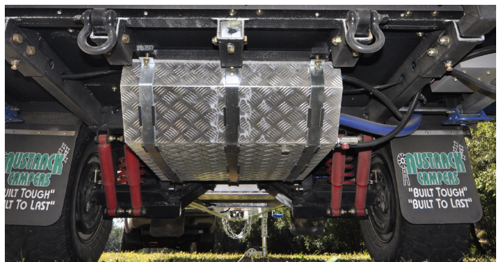
Water storage: 100L Foodgrade stainless steel water tank with aluminium tank guard & 12v pump plumbed to kitchen.
